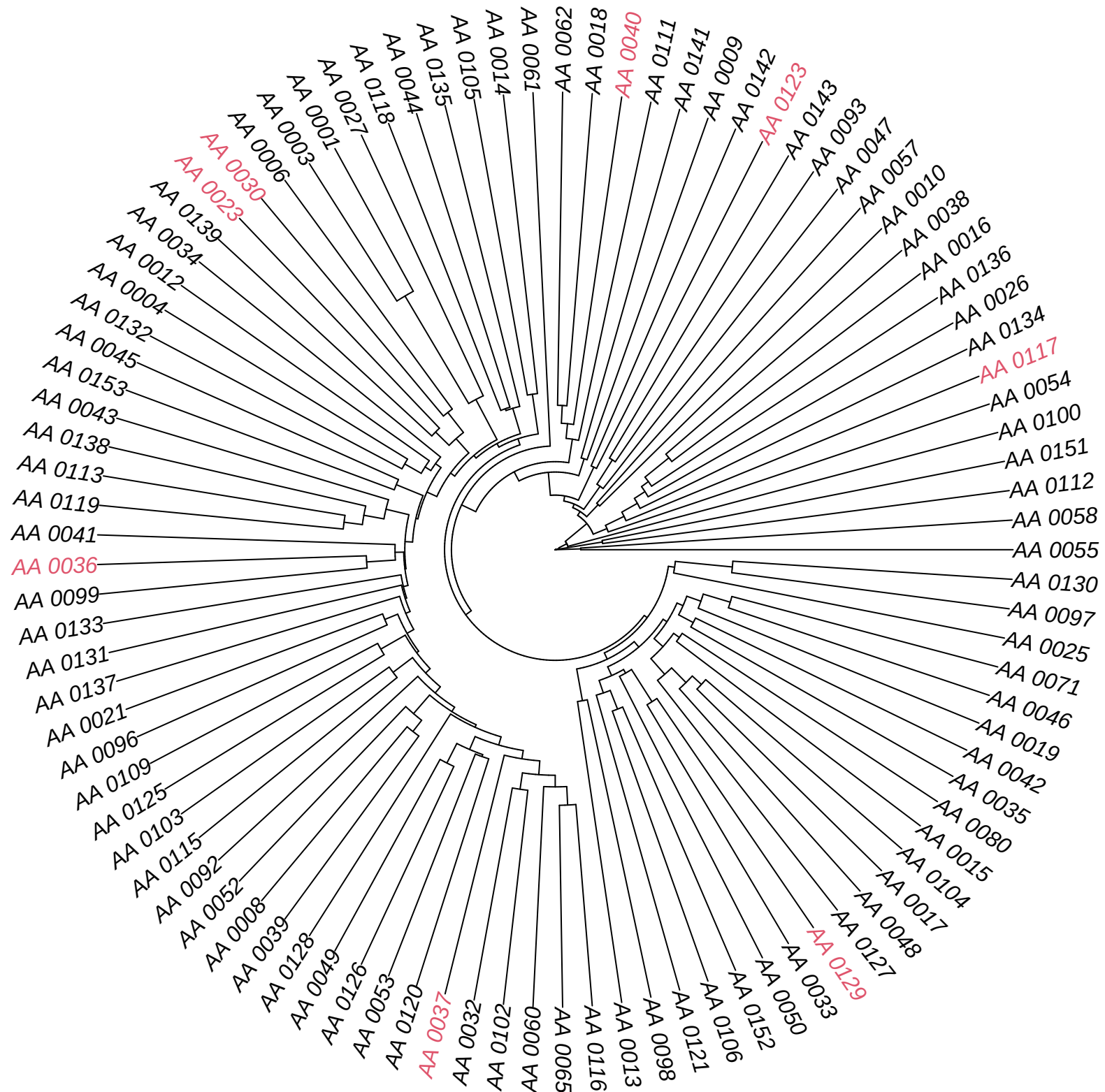
UPGMA Tree (Bray-Curtis) by Sulphonylurea
